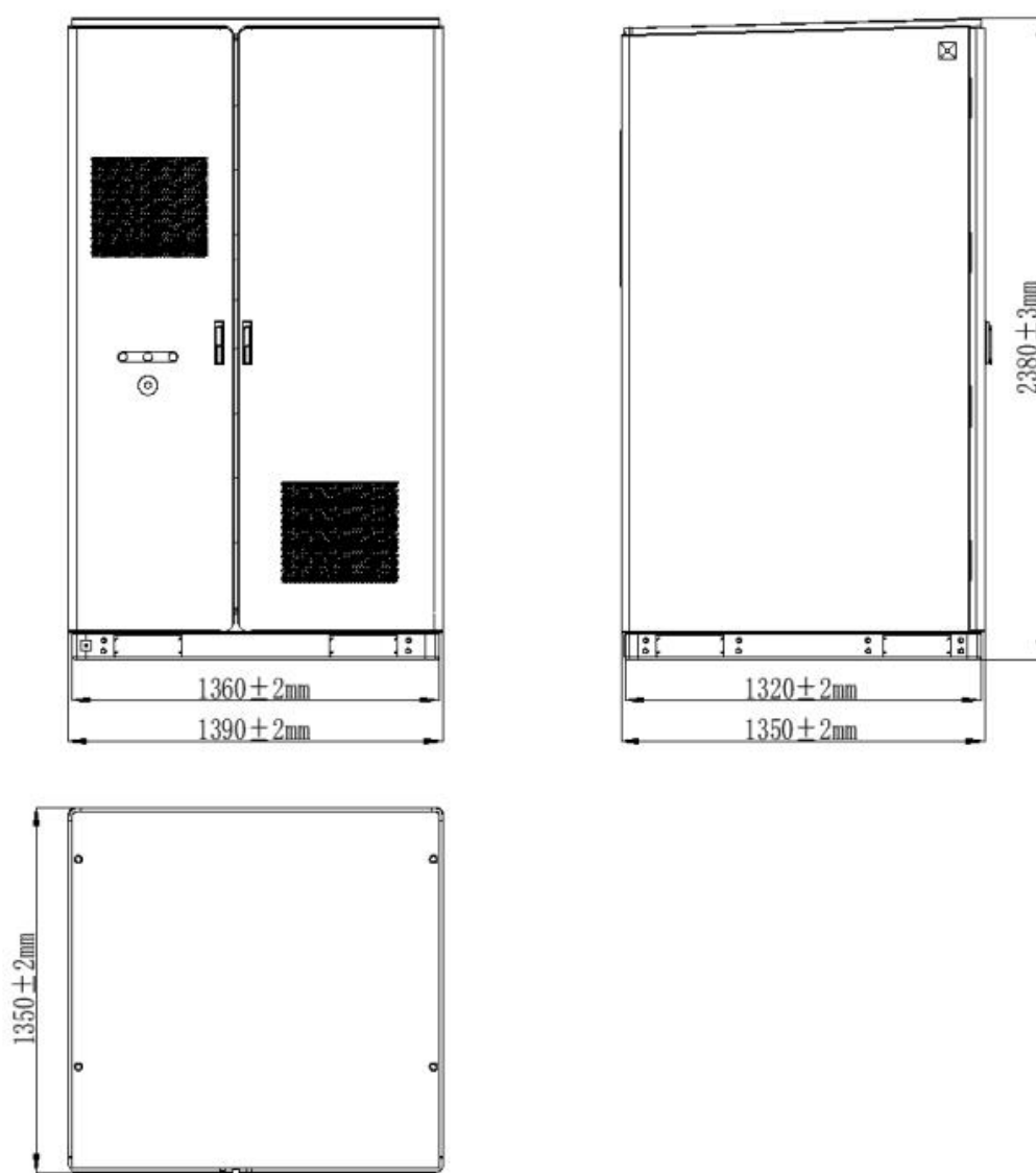
Figure 2-1 PCC dimensions
