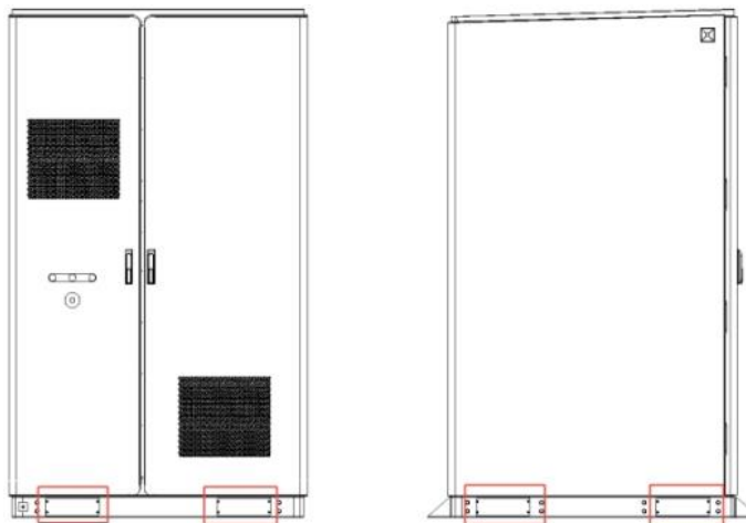
Figure 3-5 Bottom pallets position
