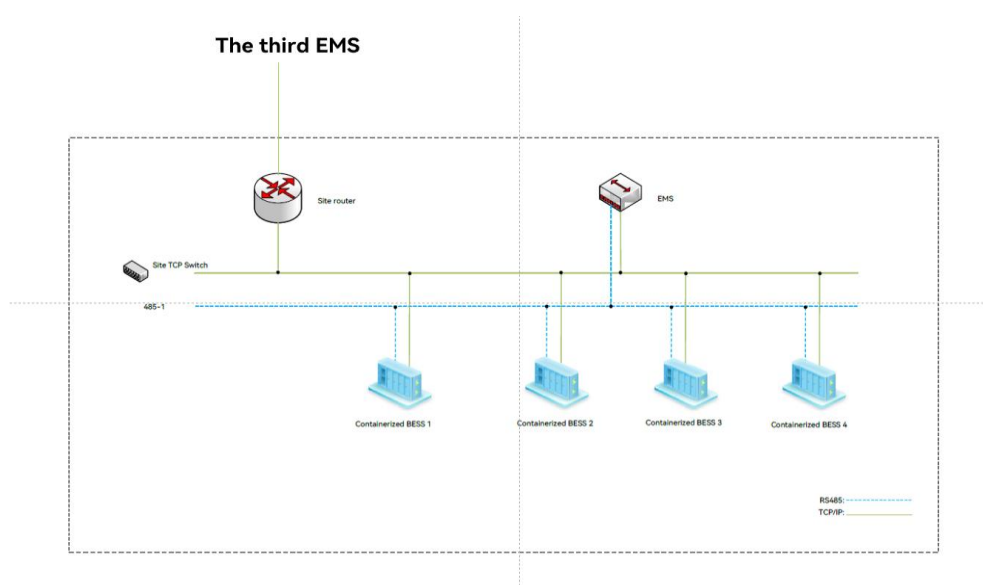
Figure 1-1 Communication Overview
